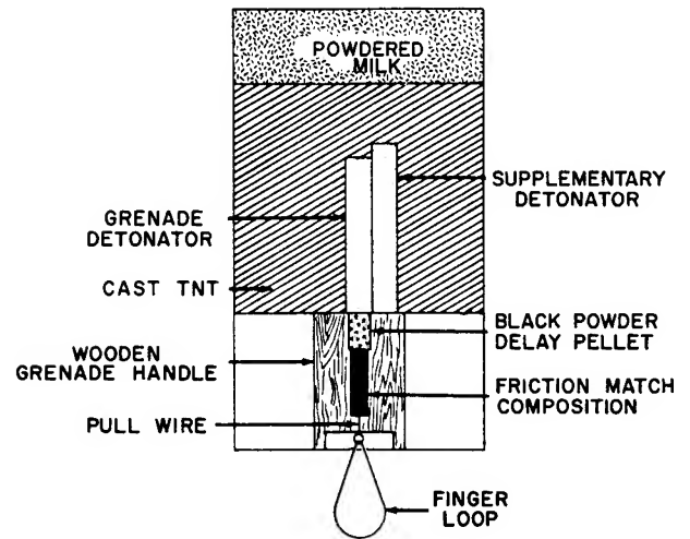
Figure 46. Milk can hand grenade.
